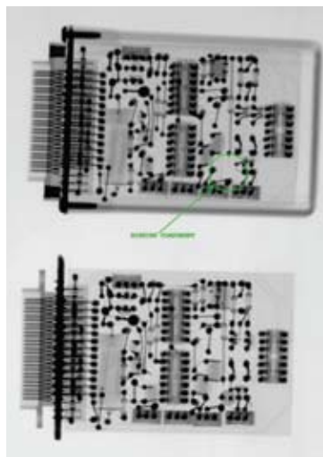
Electrical Components in Assemblies
